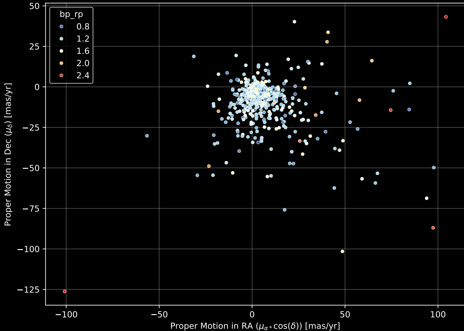
GALAH DR4 Field: [6592] Proper Motion Diagram (n= 453)
