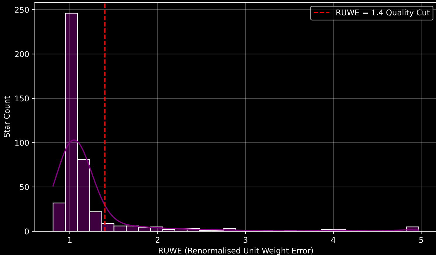
GALAH DR4 Field [6592] RUWE Distribution (n= 438)
