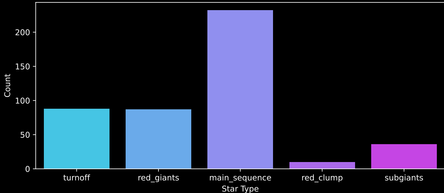
GALAH DR4 Field: [6592] Count plot of Star Type
