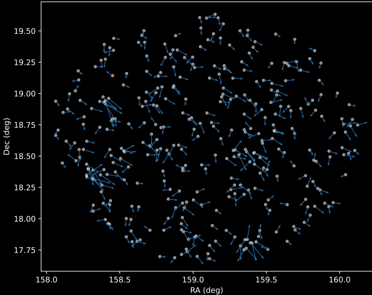
GALAH DR4 Cluster 0 Proper Motion Vectors (n=344)
