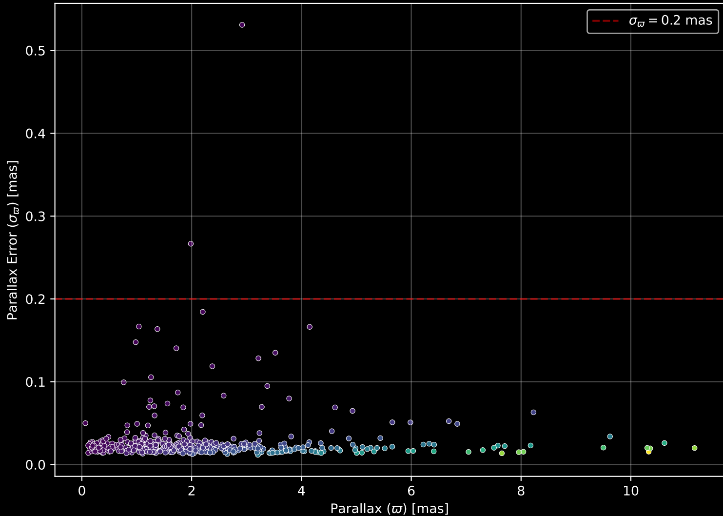
GALAH DR4 Field: [6592] Parallax Quality (n= 453)
