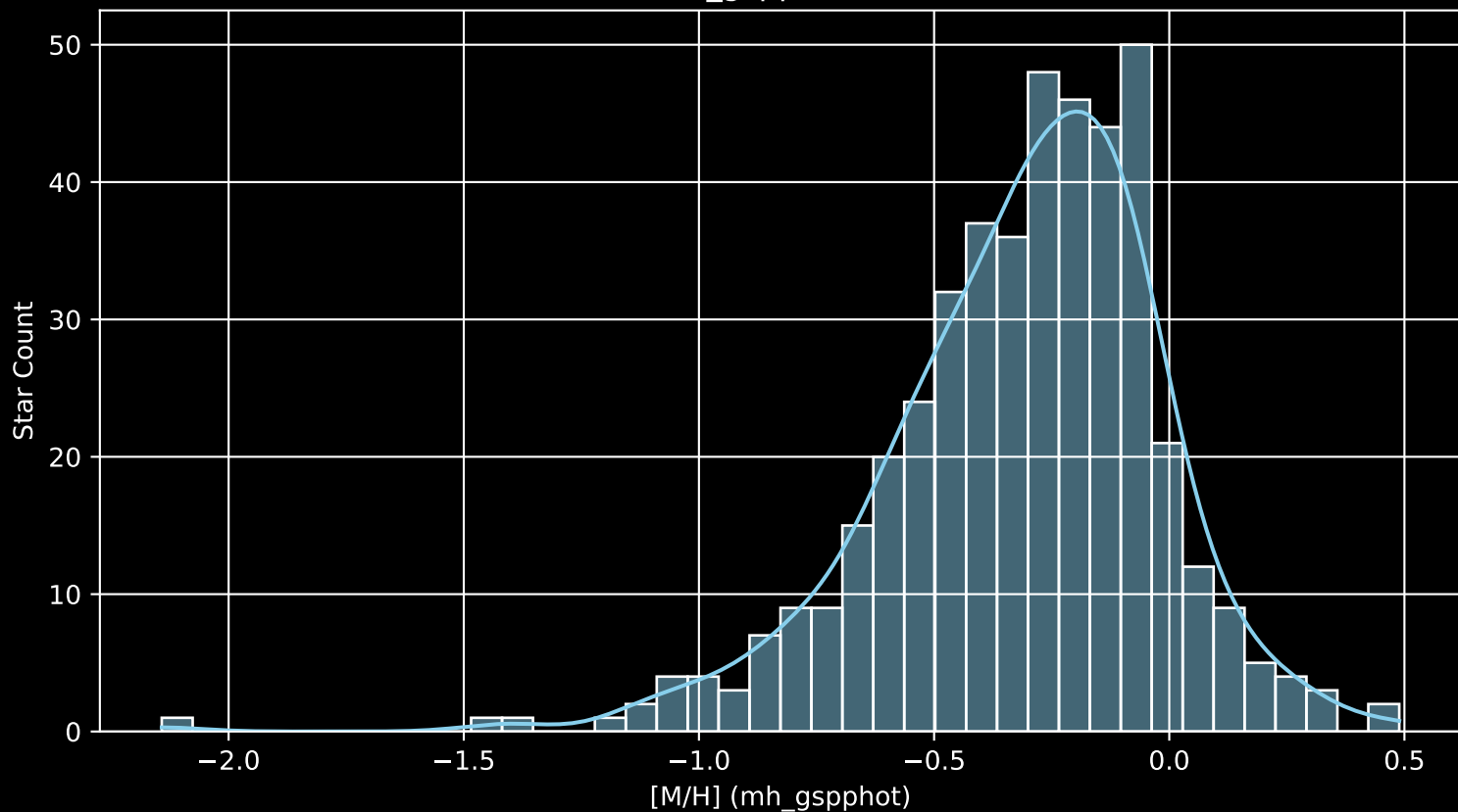
GALAH DR4 Field: [6592] [M/H] (mh_gspphot) (n= 450)
